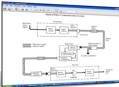
Optical Fibre Communication System
