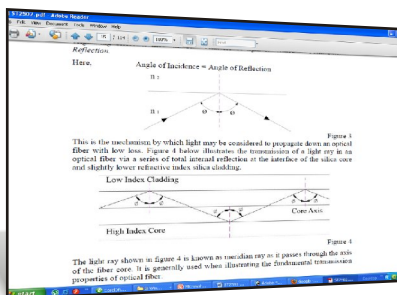
Total Internal Reflection
