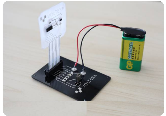
Antenna PCB
