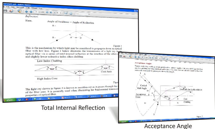
Principle of operation of Optical Fibre
