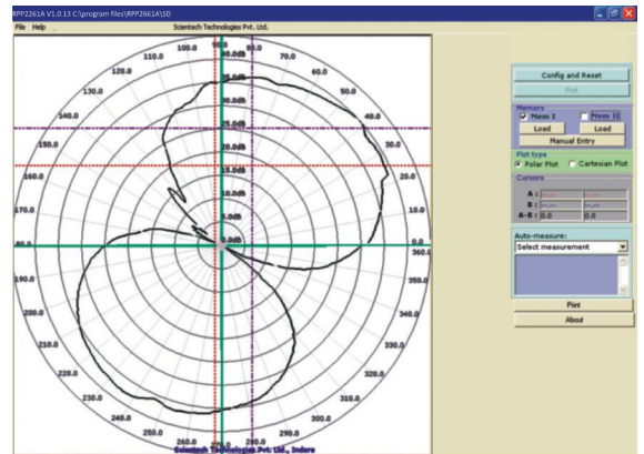
Radiation Pattern for Yagi Antenna
